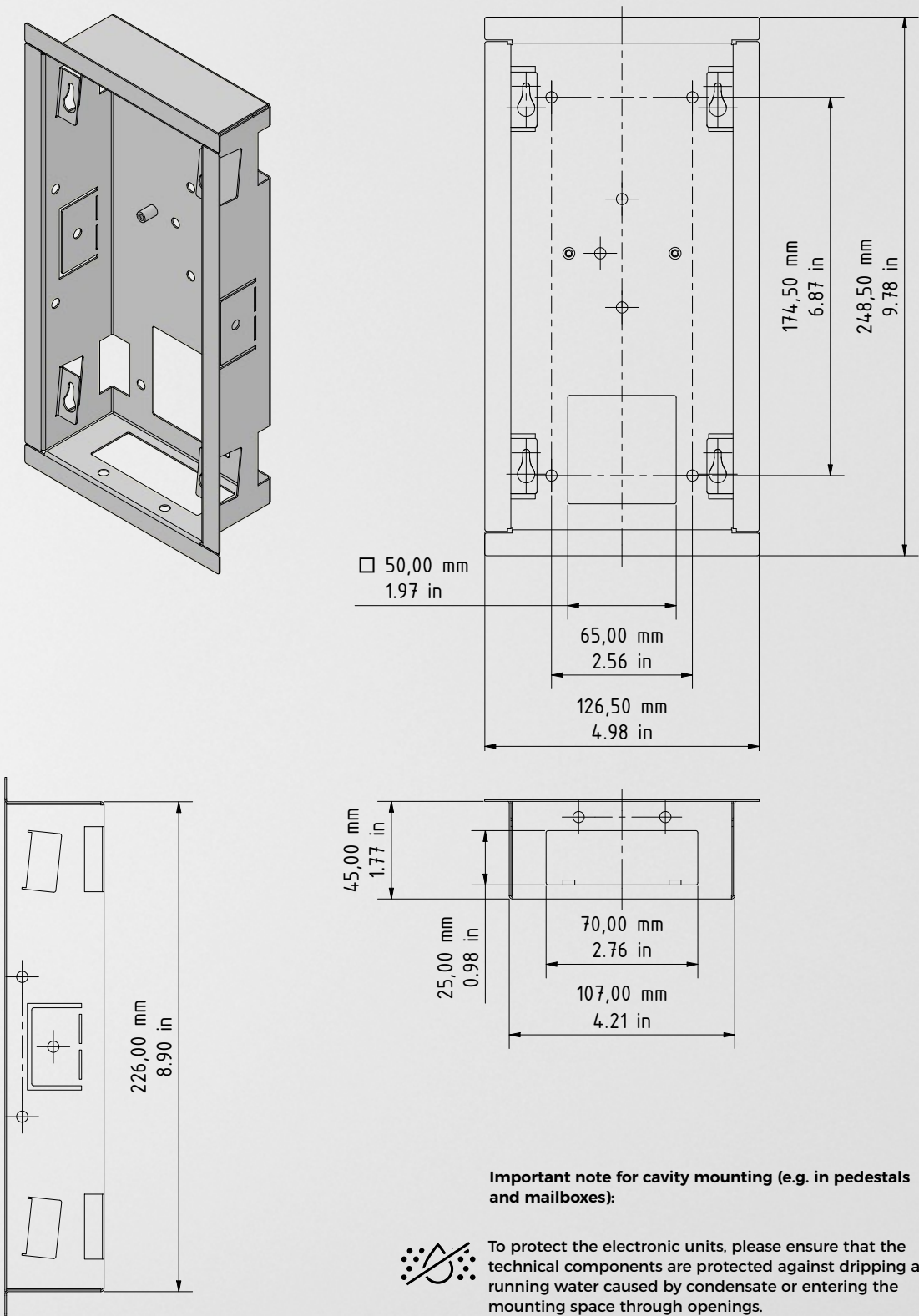
D2101V/D2201V Flush-mounting housing (backbox)
